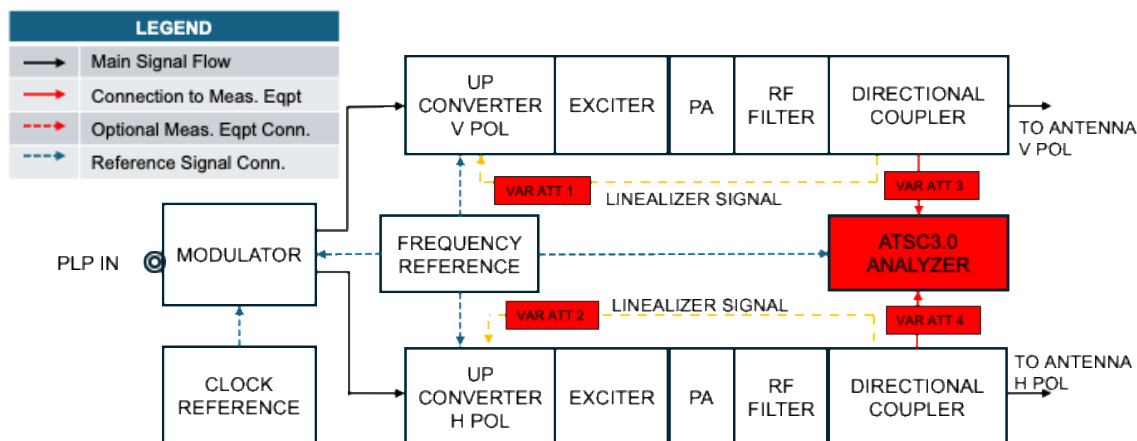
Figure A 5 – Performance Tests Setup.
