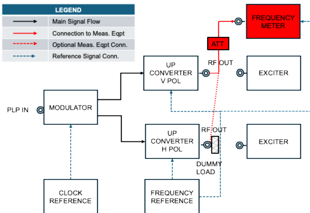
Figure A 2 – RF frequency accuracy and stability test setup.
