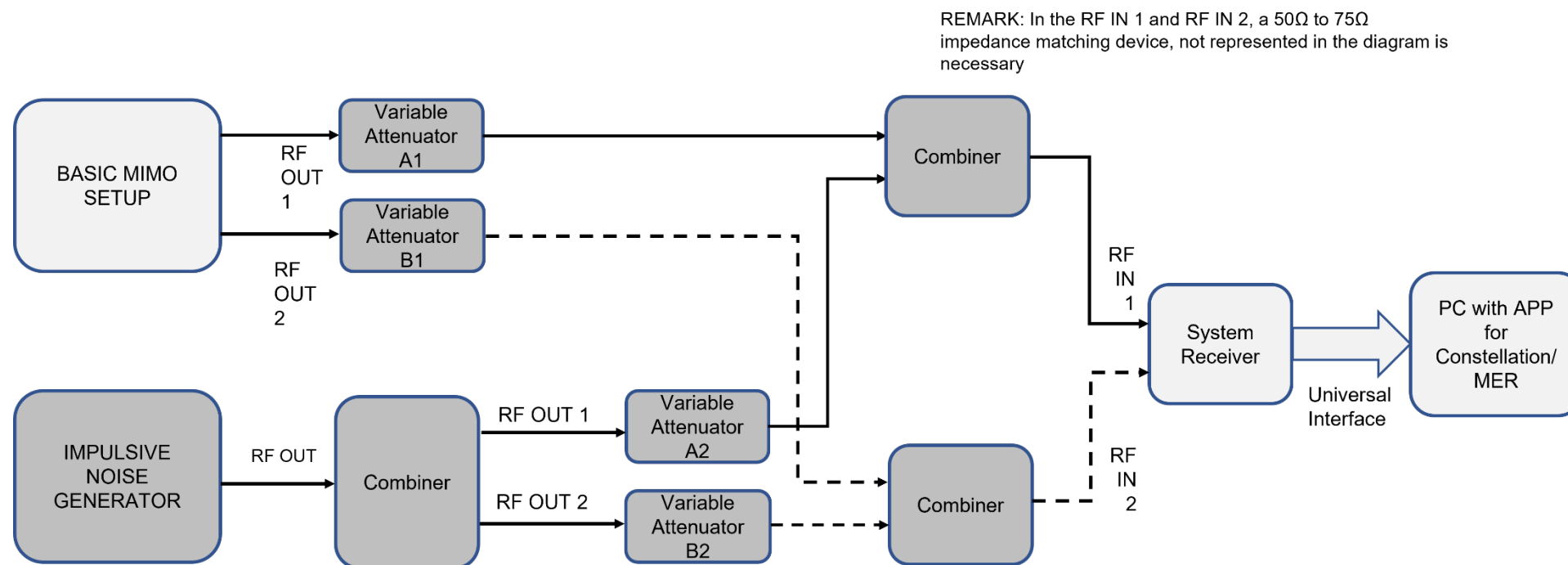
Figure 5 - Test setup for Impulsive Noise
