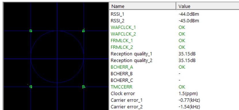
Figure A 15 - CH30 Constellation of Modulator/Demodulator A for Config 1
